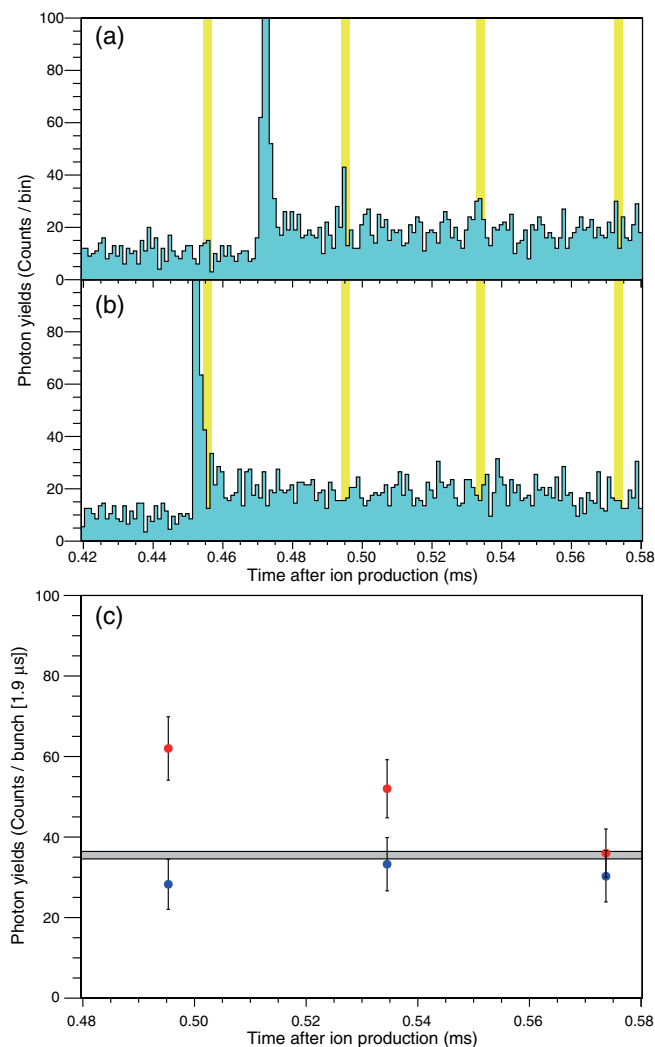
FIG. 4. RF from the photoexcited ions. (a) Temporal profile of the observed photon yield after photoexcitation (synchronized). The bin width is 1\ \mu\text{s} . The intense peak at the time of laser irradiation (approximately 0.475\ \text{ms} after ion production) is due to stray laser light. The photon emission time expected from the ion bunch timing and width ( 1.9\ \mu\text{s} ) are shown by the yellow regions. (b) Observed temporal photon yield after laser irradiation half a turn out of phase with the ion motion (countersynchronized). The peak position of the stray laser light shifts correspondingly by the time the ions undergo a half of a revolution. (c) Integrated yields at the ion bunch regions for both synchronized and countersynchronized cases are represented by red filled circles and blue filled circles, respectively.
