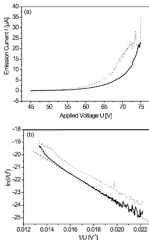
FIG. 2. (a) Measured field emission current as a function of applied voltage for two voltage scans on the same nanotube (first scan, dotted; second scan, full line). (b) The corresponding Fowler-Nordheim plot.
