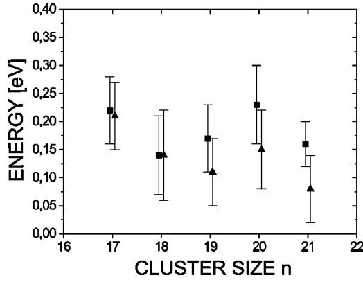
FIG. 5. Left hand side of Eq. (13) (squares) and E_{KER,n}(n,n-3) - E_{KER,n}(n,n-2) (triangles) as a function of cluster size. The error bars on the kinetic-energy release difference represent the estimated systematic value, while those of the photoexcitation energies are derived from the measured shifts.
