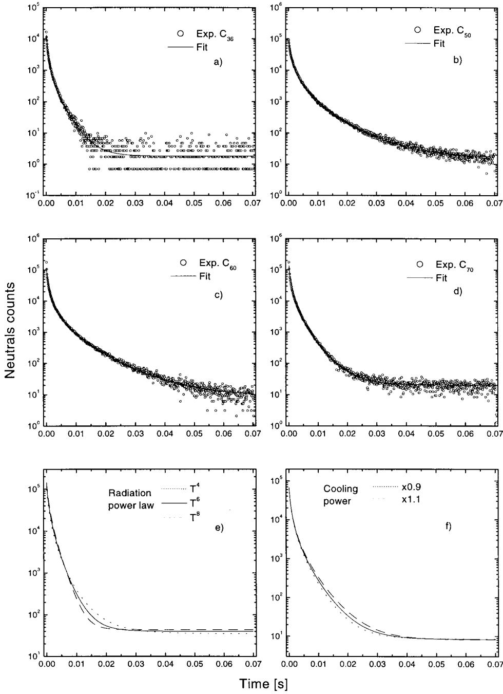
Fig. 9. As Figure 8 but for the magic fullerene anions C_N^- , N = 36, 50, 60 , and 70 . The two lower curves illustrate the sensitivity of the simulations to a variation of the cooling power and its temperature dependence.
