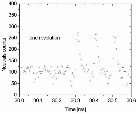
Fig. 4. Section of a time spectrum for C_{60}^- stored in ELISA and exposed at \sim 30.3 ms after injection to a 2 mJ laser pulse with 1.2 eV photon energy. The points correspond to 5 \mu s intervals and the revolution time is about 100 \mu s .
