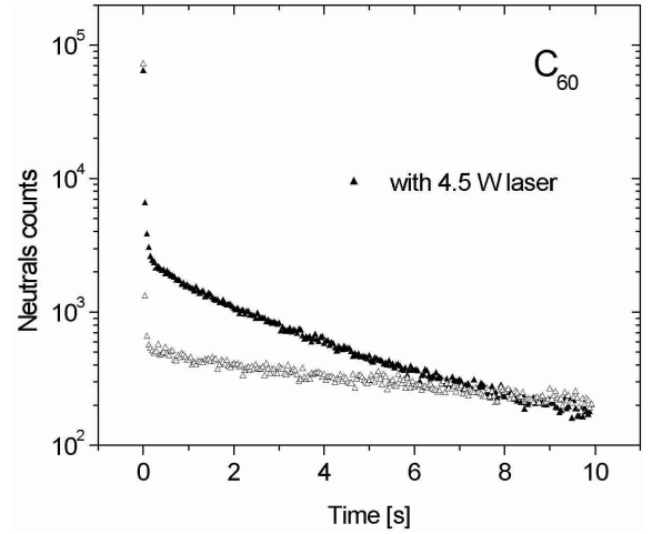
Fig. 3. Time spectrum of neutrals counts for a stored C_{60}^- beam in ELISA, with and without irradiation by a 4.5 W CW Nd:YAG laser. Each point corresponds to a 40 ms interval.
