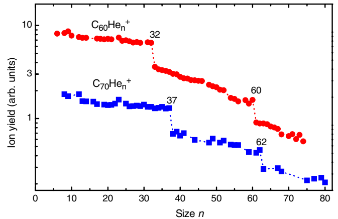
FIG. 2 (color online). Ion yields of ^{12}\text{C}_{60}\text{He}_n^+ and ^{12}\text{C}_{70}\text{He}_n^+ versus size n .
